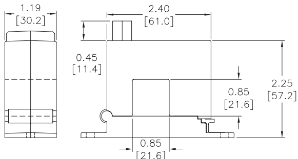
ACSL Series Split Core
