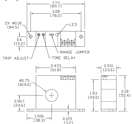
ACSX Series Fixed Core
