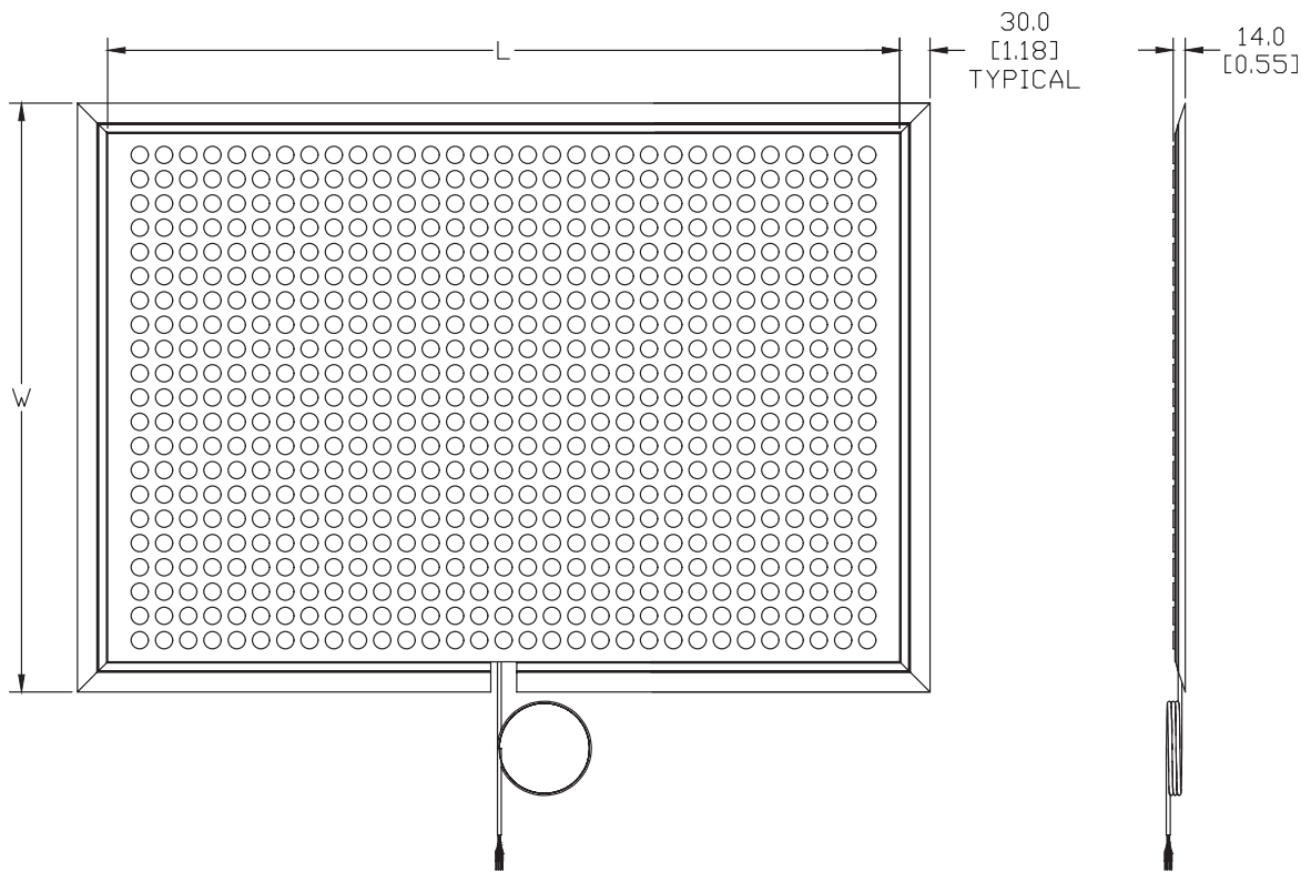
Contact Mats - Tapered Edge (1602-4XXX)
