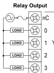
Relay Output Wiring Diagram
