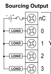
Output Wiring Diagram
