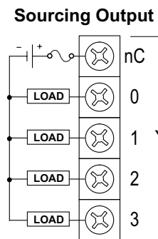
Output Wiring Diagram
