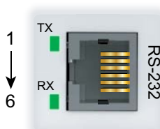
6-pin RJ12 Female Modular Connector
