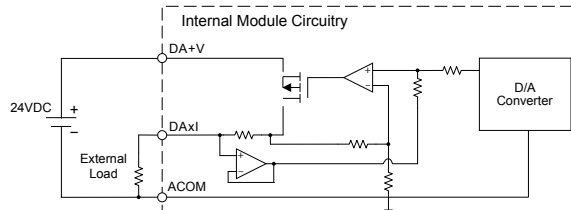
Analog Current Output Circuit
