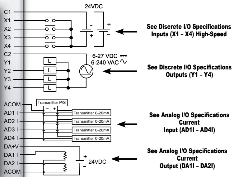
Wiring Diagram
