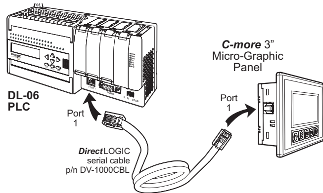
C-more 3-inch Micro Port 1 to DL06 PLC Port 1
