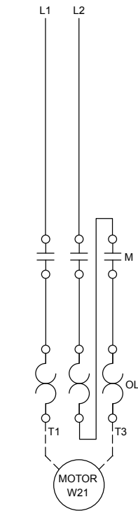
NON COMBINATION 1-PHASE
