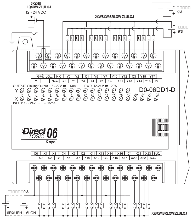
Equivalent input circuit, Standard inputs (X4-X23)
