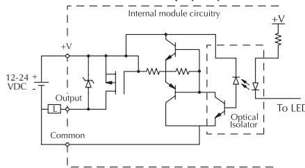
Equivalent output circuit Pulse output (Y0-Y1)
