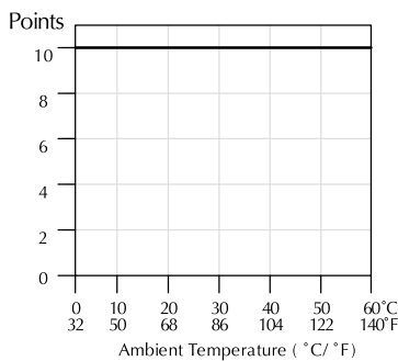
Derating chart for AC inputs
