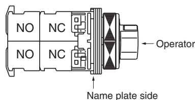
4- and 5-pos Contact Positions
