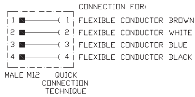
4-Pole Male Connector
