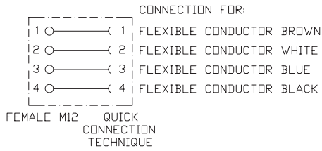
4-Pole Female Connector
