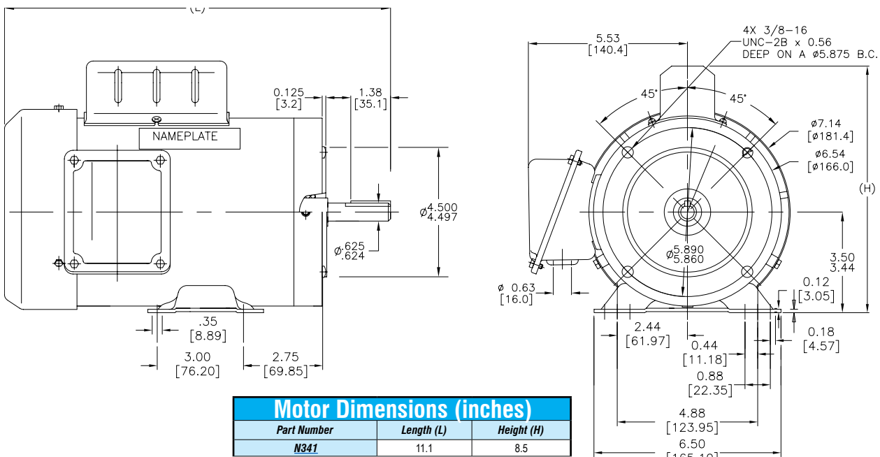
Figure 1 - N341 Dimensions
