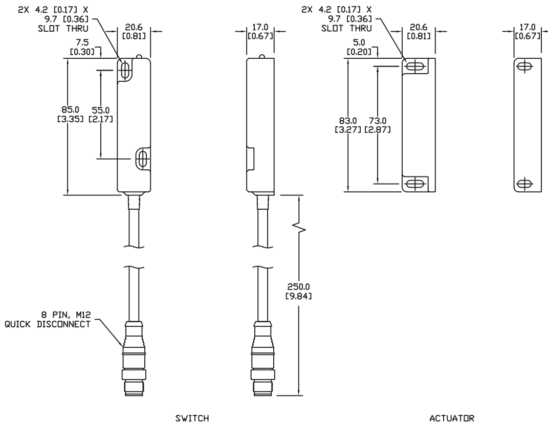
Quick Disconnect
