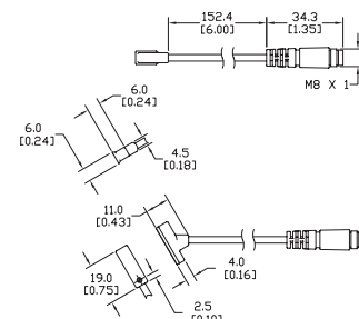
CPS9D-xx-F cable length tolerance ± 1.5"
