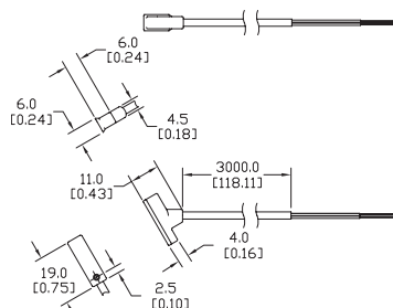
CPS9D-xx-A wire length tolerance +12" / - 0"
