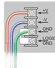
12-24 VDC
