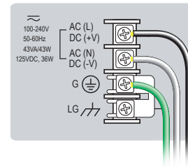
P2-01DCAC
