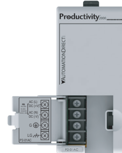
P2-01AC
