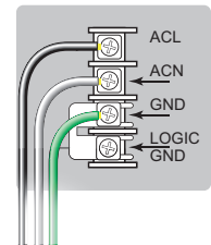
24VAC
