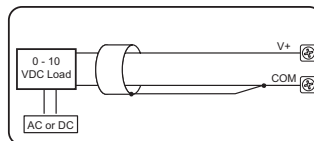
Voltage Output
