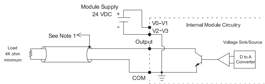
Equivalent Output Circuit
