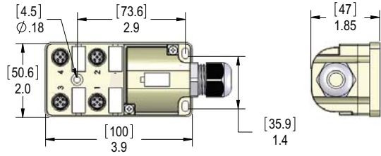
Figure 1: 4 Port 4 Pin
