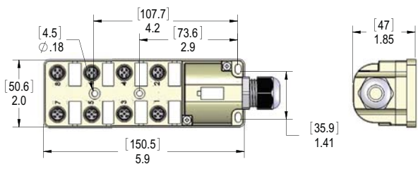
Figure 5: 8 Port 4 Pin
